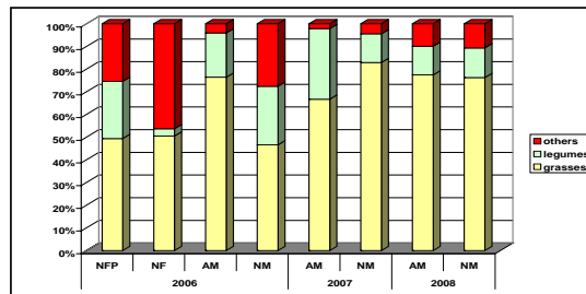
Figure 1: botanical composition in % in the new an control pastures
